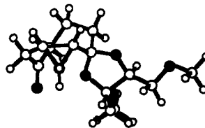
conformer 40
