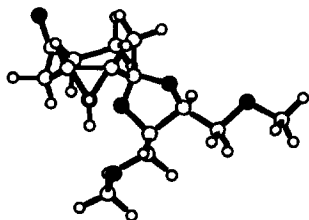
conformer 11
